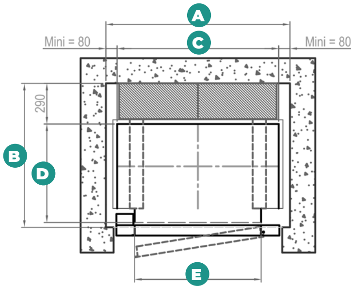
Gaine Sheat
