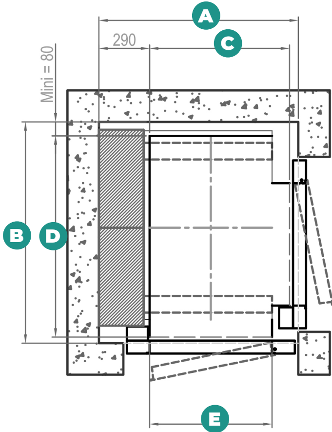
Gaine Sheath
