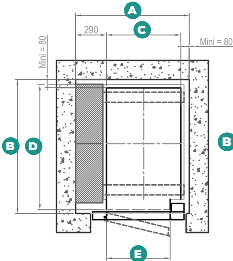
Gaine Sheat
