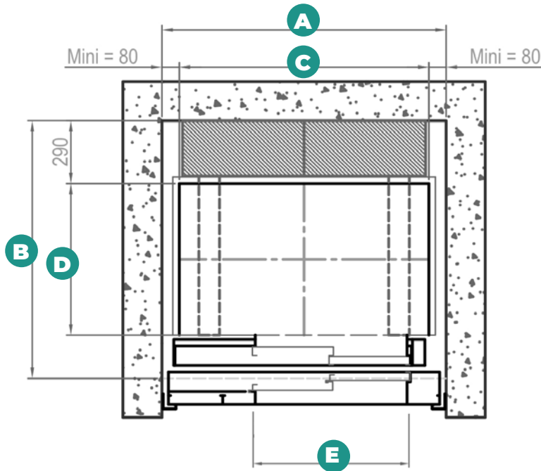
Gaine Sheat
